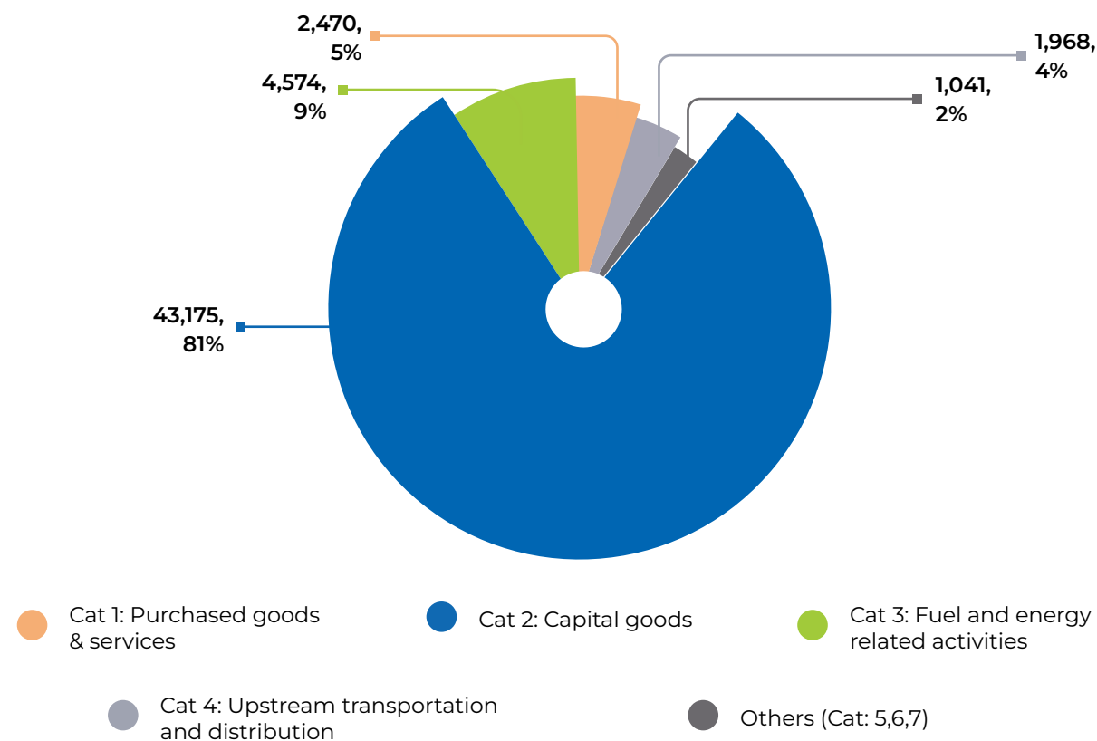
Contribution of Scope 3 Emissions by Category (tCO 2 e, % contribution)
